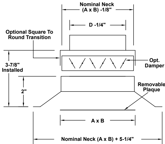
SURFACE MOUNTED
