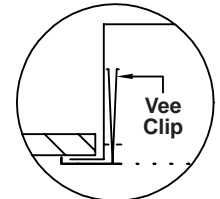
REMOVABLE FACE CLIP DETAIL (Surface Mount Only)
