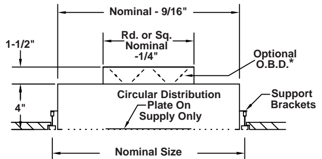
FOR SPECIAL 9/16" WIDE T-BAR CEILINGS - STYLE C
