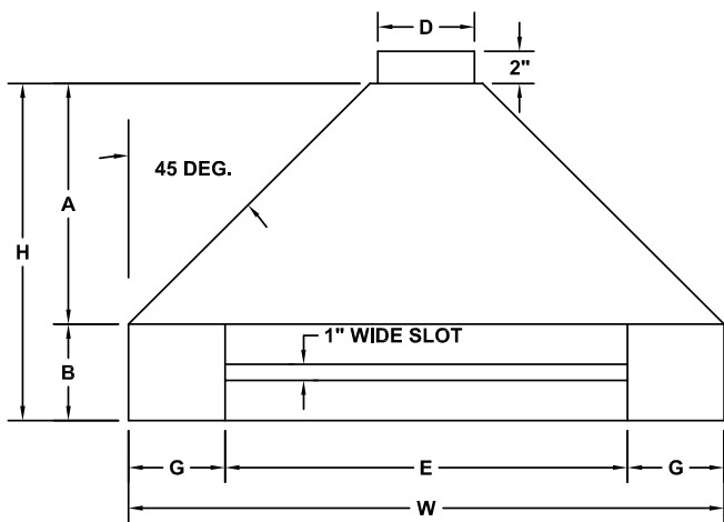
ELEVATION VIEW
