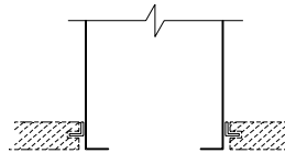
Option 17 Splined Ceiling "K" Diffusers Only
