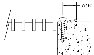
MOUNTING OPTION A #8 SCREWS WITH COUNTERSUNK HOLES
