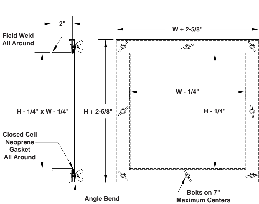
FLAT DUCT MODEL UHPA
