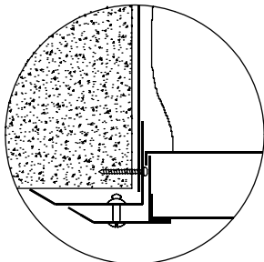
SURFACE MOUNT
