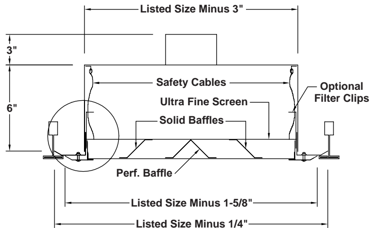
SURFACE MOUNT
