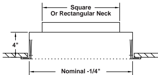
SURFACE MOUNT - STYLE B (Return) Removable Face
