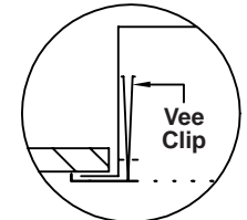
REMOVABLE FACE CLIP DETAIL (Surface Mount Only)
