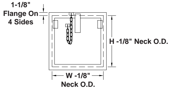
Optional 1" or 2" Double Wall Insulation
