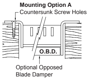
COUNTERSUNK SCREW HOLES / OPPOSED BLADE DAMPER
