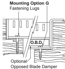
FASTENING LUGS / FASTENING LUGS WITH OPPOSED BLADE DAMPER
