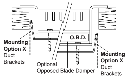
DUCT BRACKETS / DUCT BRACKETS WITH OPPOSED BLADE DAMPER
